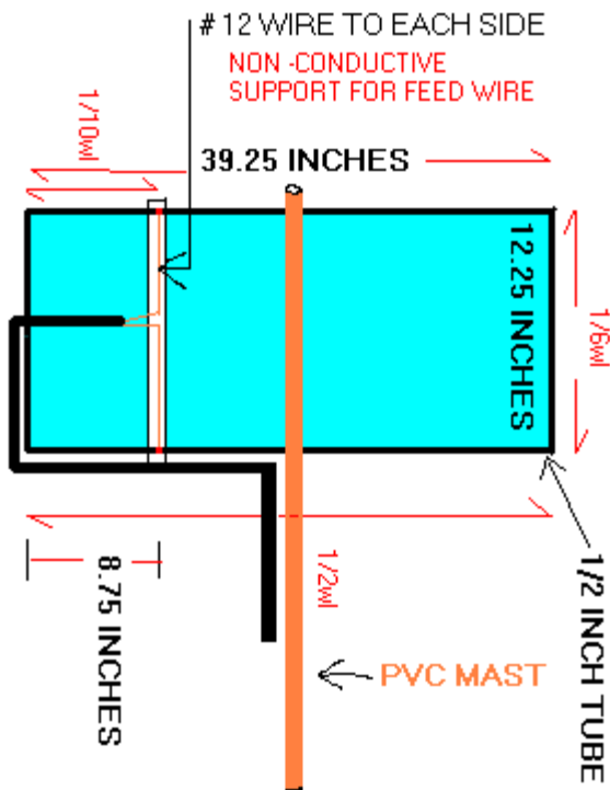
Drawing not to scale!
